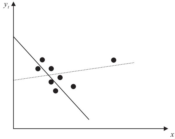
Figure 4.13 Possible effect of an outlier on OLS estimation
