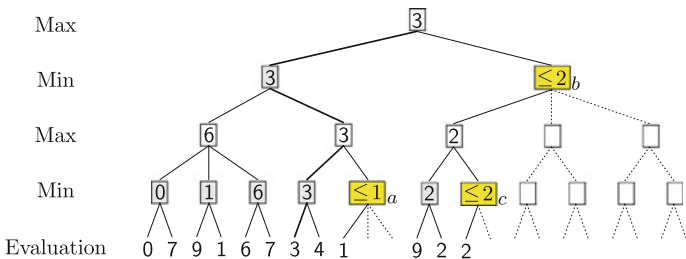
Fig. 6.20 An alpha-beta game tree with look-ahead of four half-moves. The dotted portions of the tree are not traversed because they have no effect on the end result
