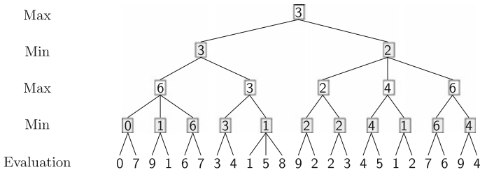
Fig. 6.19 A minimax game tree with look-ahead of four half-moves
