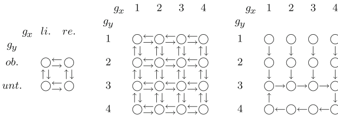
Fig. 10.3 The state space of the example robot in the case of two possible positions for each of the joints ( left ) and in the case of four horizontal and vertical positions for each ( middle ). In the right image an optimal policy is given
