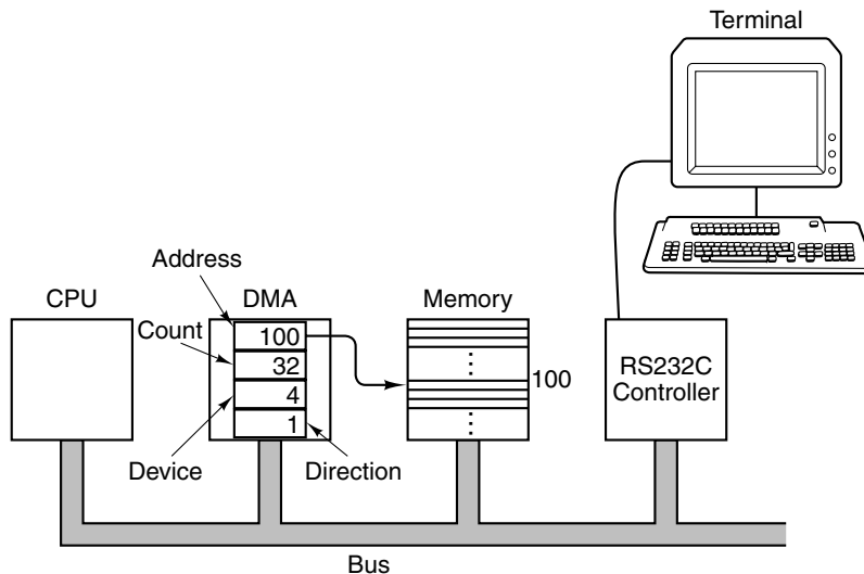
Figure 5-33. A system with a DMA controller.
