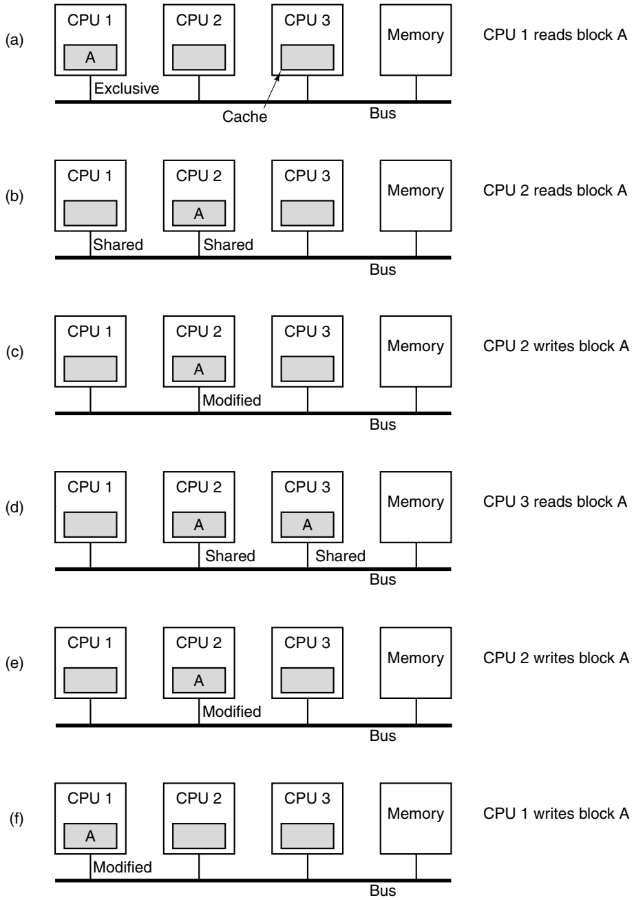
Figure 8-26. The MESI cache coherence protocol.
