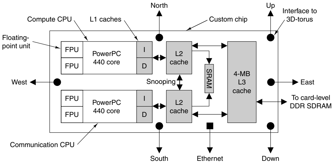
Figure 8-36. The BlueGene/L custom processor chip.
