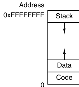
Figure 6-32. The address space of a single UNIX process.
