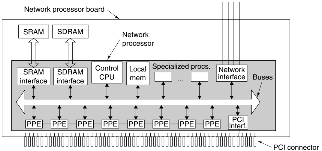
Figure 8-15. A typical network processor board and chip.
