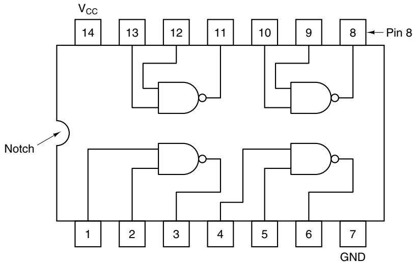
Figure 3-10. An SSI chip containing four gates.
