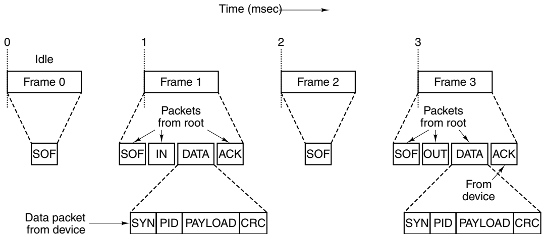
Figure 3-59. The USB root hub sends out frames every 1.00 msec.
