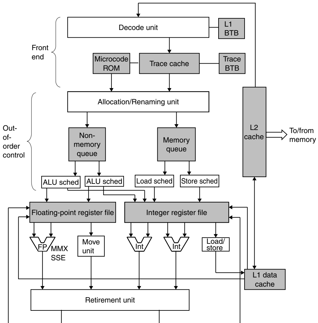
Figure 4-47. A simplified view of the Pentium 4 data path.
