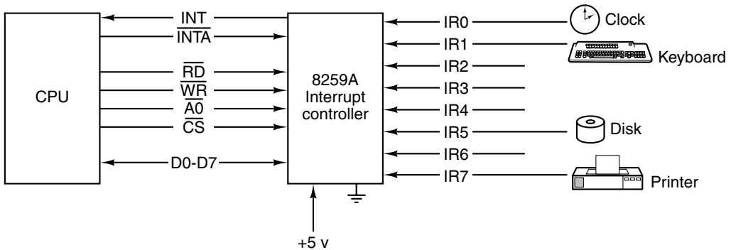
Figure 3-43. Use of the 8259A interrupt controller.
