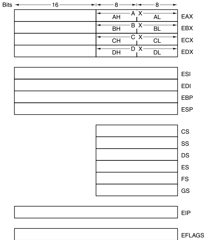
Figure 5-3. The Pentium 4's primary registers.
