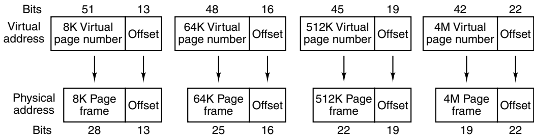
Figure 6-17. Virtual to physical mappings on the UltraSPARC.
