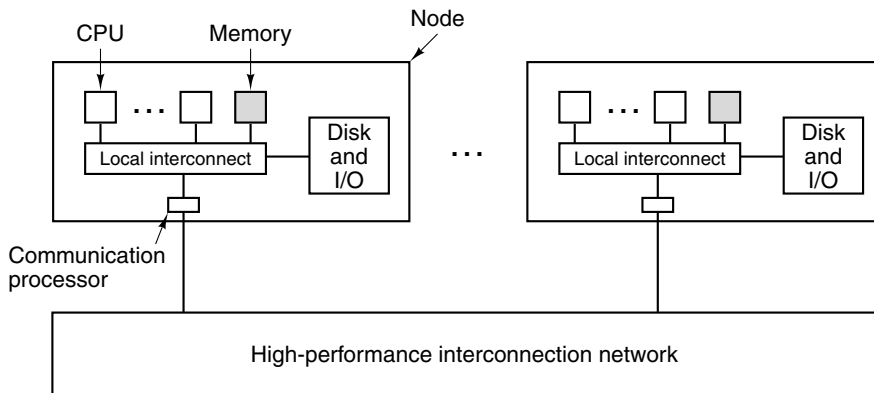
Figure 8-34. A generic multicomputer.
