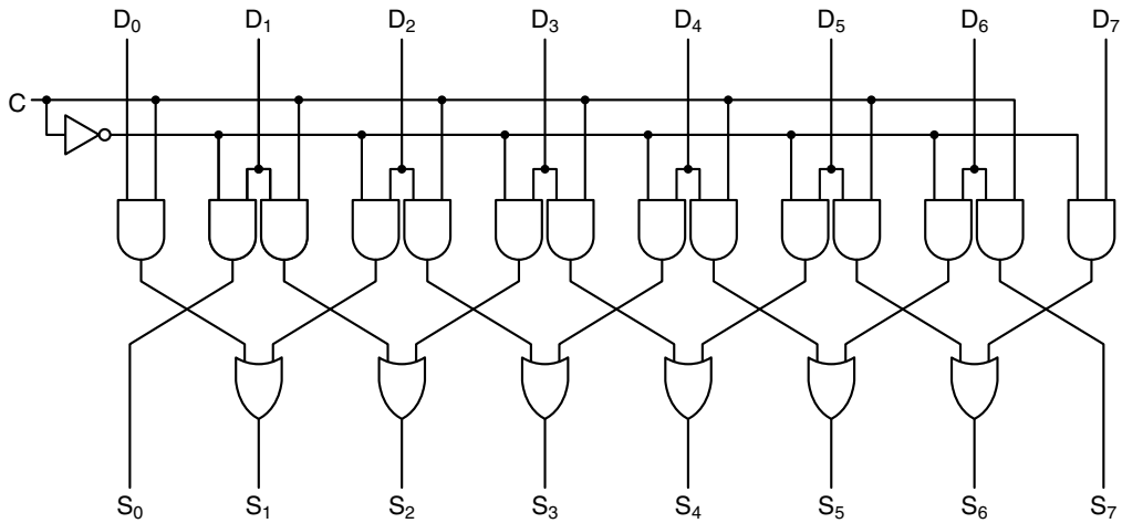
Figure 3-16. A 1-bit left/right shifter.
