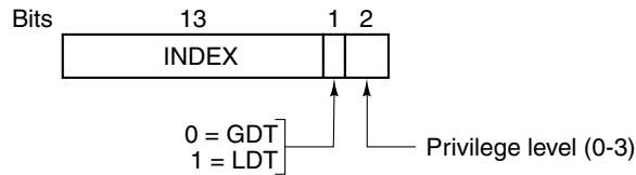
Figure 6-12. A Pentium 4 selector.
