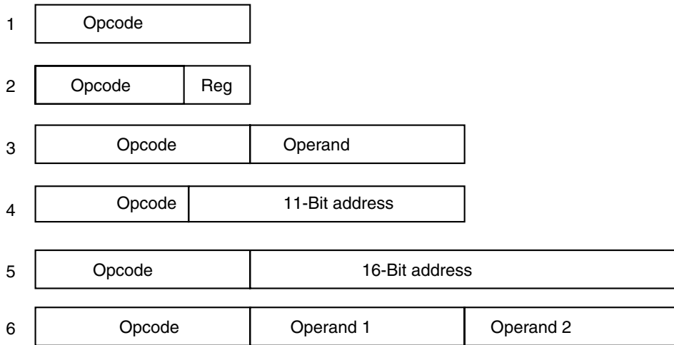
Figure 5-16. The 8051 instruction formats.
