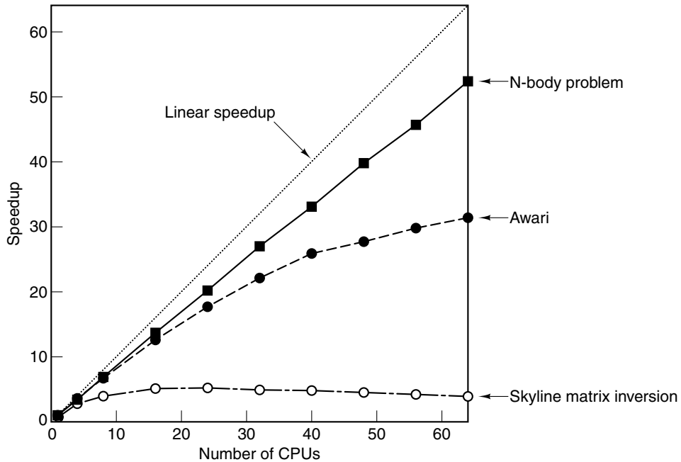
Figure 8-47. Real programs achieve less than the perfect speedup indicated by the dotted line.
