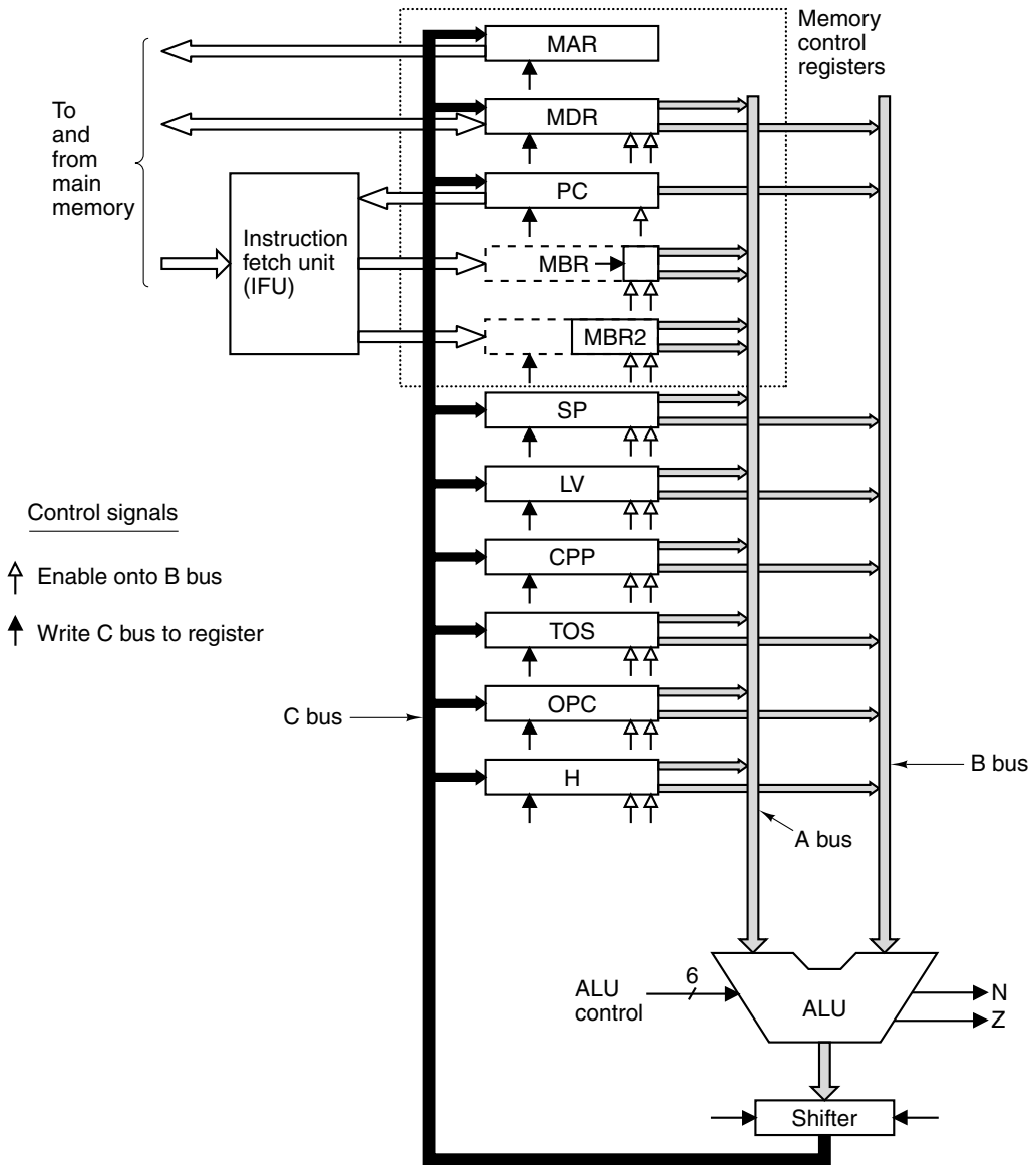
Figure 4-29. The datapath for Mic-2.
