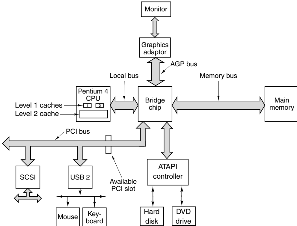
Figure 3-53. The bus structure of a modern Pentium 4.
