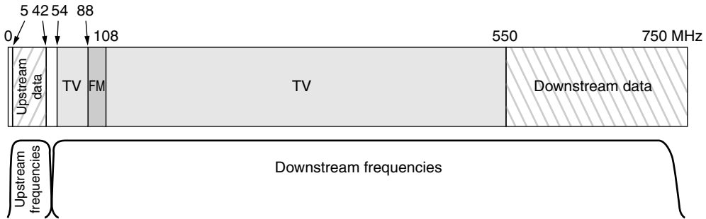
Figure 2-40. Frequency allocation in a typical cable TV system used for Internet access.
