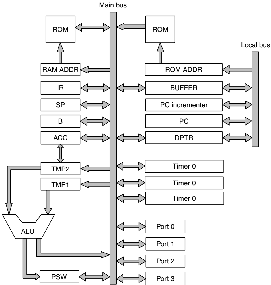
Figure 4-50. The microarchitecture of the 8051.
