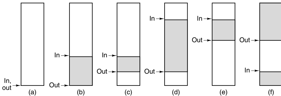
Figure 6-24. Use of a circular buffer.
