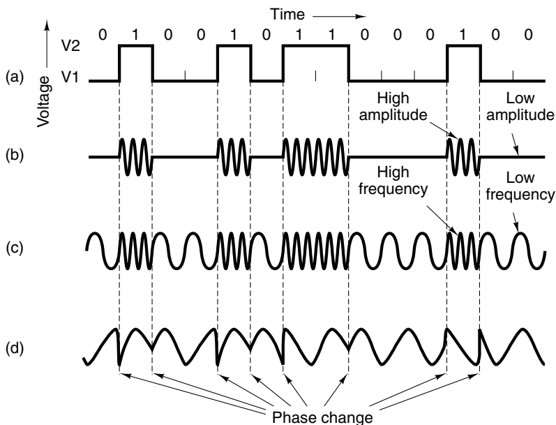
Figure 2-37. Transmission of the binary number 01001011000100 over a telephone line bit by bit. (a) Two-level signal. (b) Amplitude modulation. (c) Frequency modulation. (d) Phase modulation.
