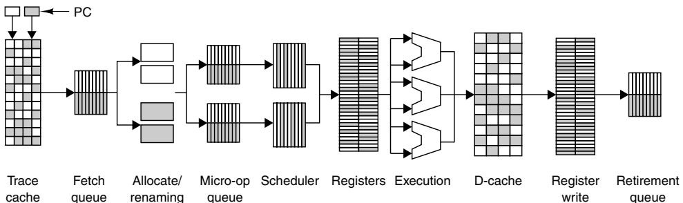
Figure 8-9. Resource sharing between threads in the Pentium 4 NetBurst microarchitecture.
