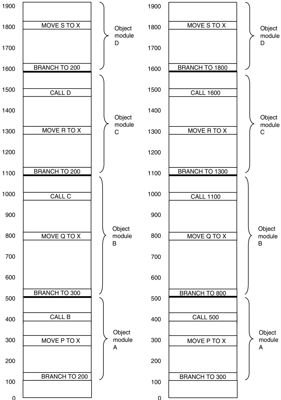
Figure 7-15. (a) The object modules of Fig. 7-14 after being positioned in the binary image but before being relocated and linked. (b) The same object modules after linking and after relocation has been performed.
