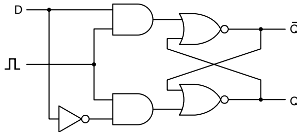
Figure 3-24. A clocked D latch.
