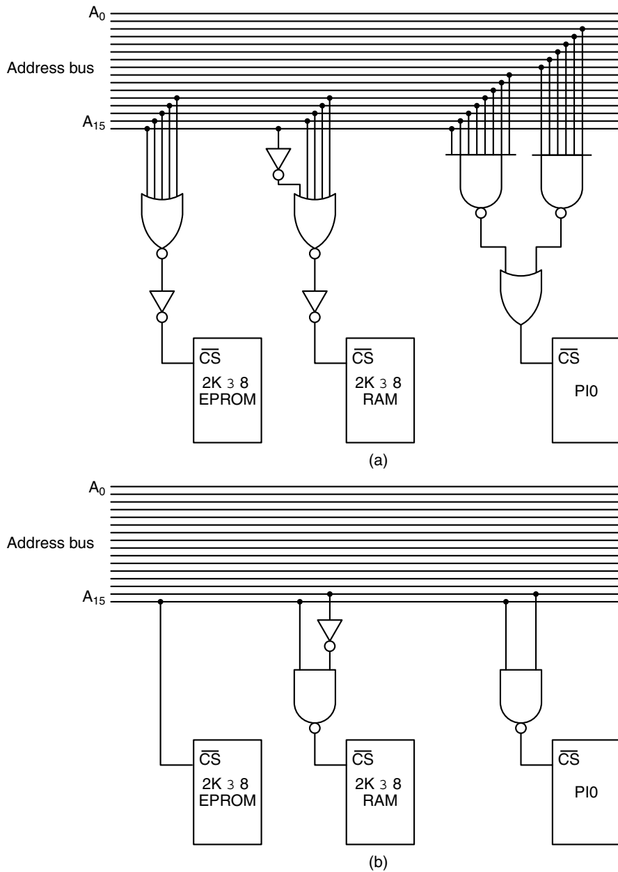
Figure 3-62. (a) Full address decoding. (b) Partial address decoding.
