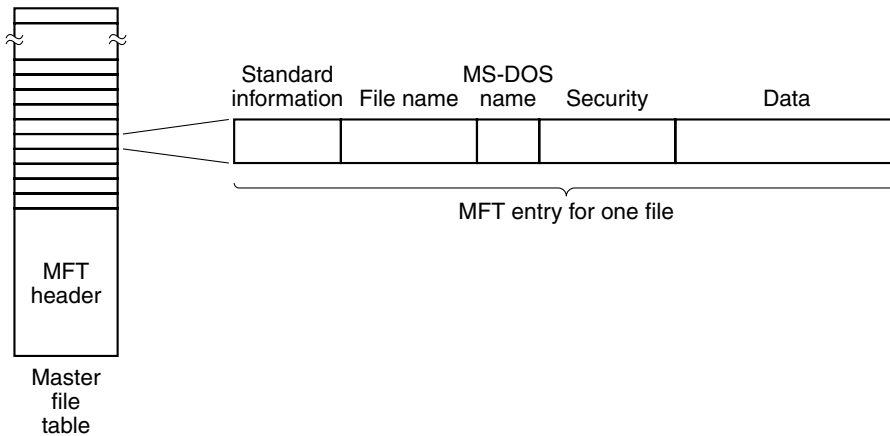
Figure 6-41. The Windows XP master file table.
