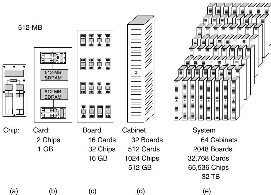
Figure 8-37. The BlueGene/L (a) chip. (b) card. (c) board. (d) cabinet. (e) system.
