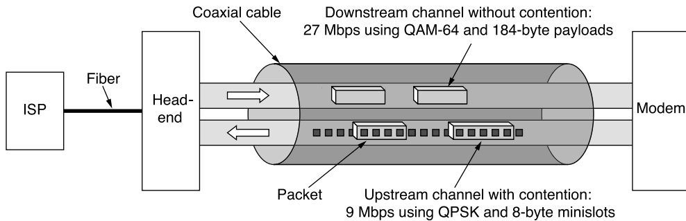
Figure 2-41. Typical details of the upstream and downstream channels in North America. QAM-64 (Quadrature Amplitude Modulation) allows 6 bits/Hz but only works at high frequencies. QPSK (Quadrature Phase Shift Keying) works at low frequencies but allows only 2 bits/Hz.
