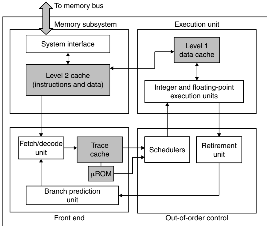
Figure 4-46. The block diagram of the Pentium 4.
