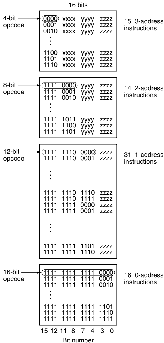
Figure 5-13. An expanding opcode allowing 15 three-address instructions, 14 two-address instructions, 31 one-address instructions, and 16 zero-address instructions. The fields marked xxxx , yyyy , and zzzz are 4-bit address fields.
