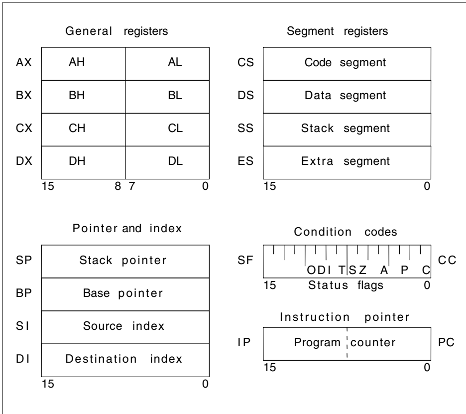
Figure C-2. The 8088 registers.
