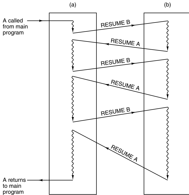
Figure 5-45. When a coroutine is resumed, execution begins at the statement where it left off the previous time, not at the beginning.
