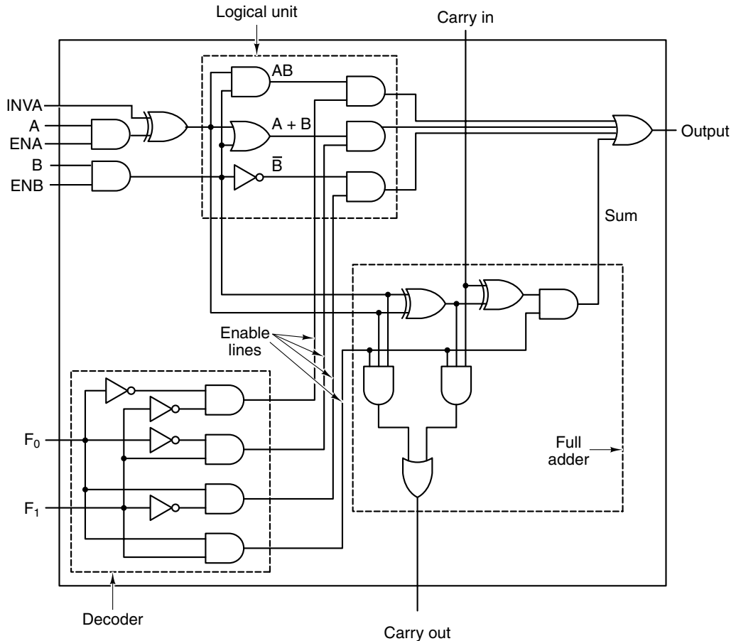
Figure 3-19. A 1-bit ALU.
