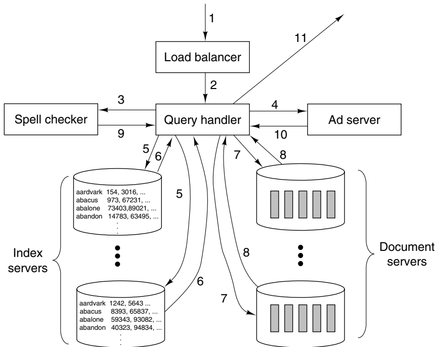
Figure 8-41. Processing of a Google query.
