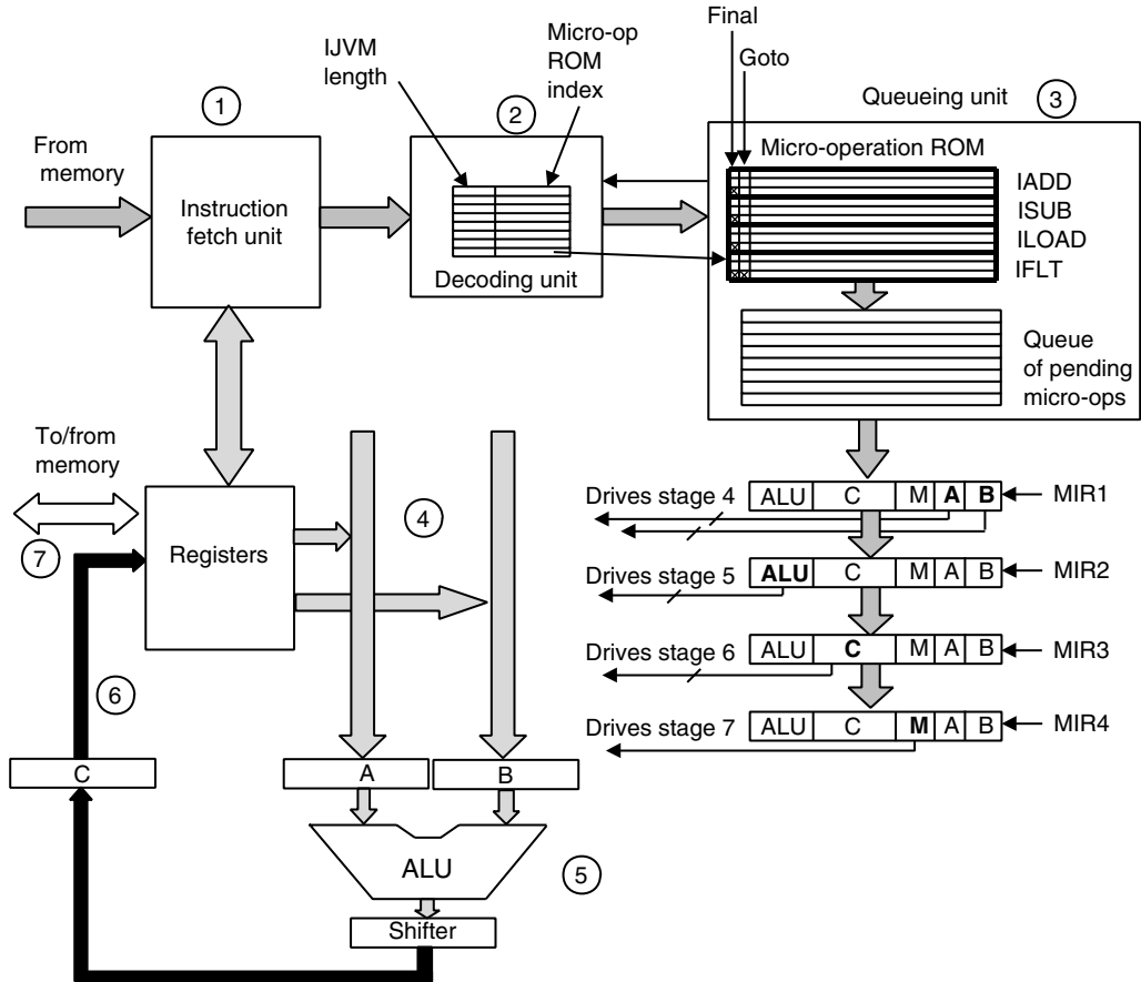
Figure 4-35. The main components of the Mic-4.
