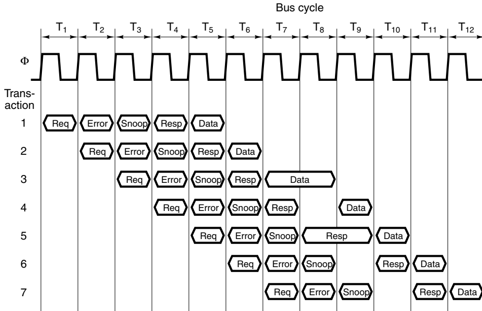
Figure 3-46. Pipelining requests on the Pentium 4's memory bus.
