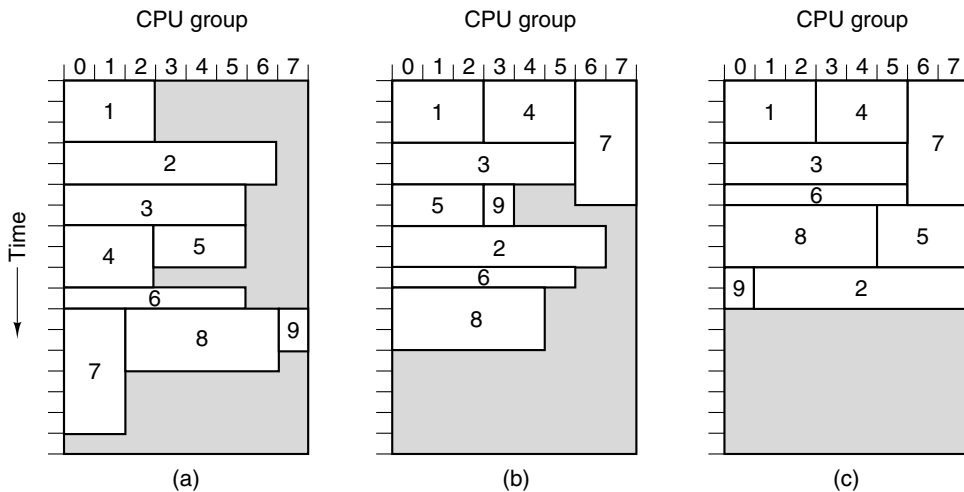
Figure 8-43. Scheduling a cluster. (a) FIFO. (b) Without head-of-line blocking. (c) Tiling. The shaded areas indicate idle CPUs.
