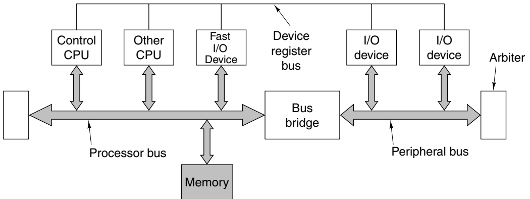
Figure 8-12. An example of the IBM CoreConnect architecture.
