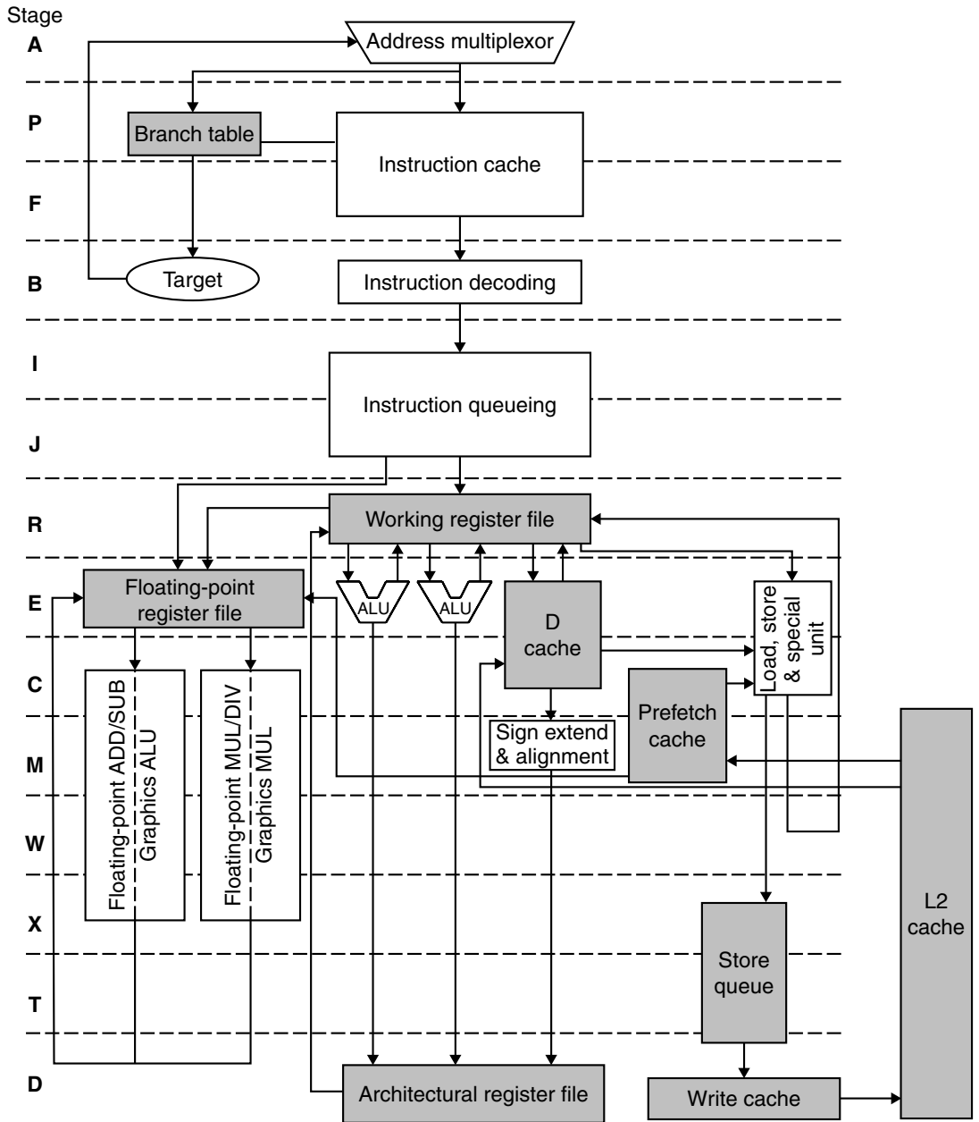
Figure 4-49. A simplified representation of the UltraSPARC III Cu pipeline.
