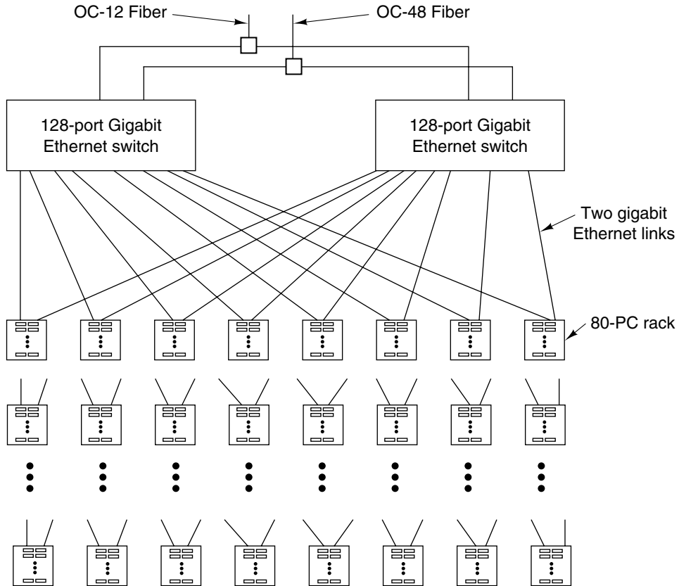
Figure 8-42. A typical Google cluster.
