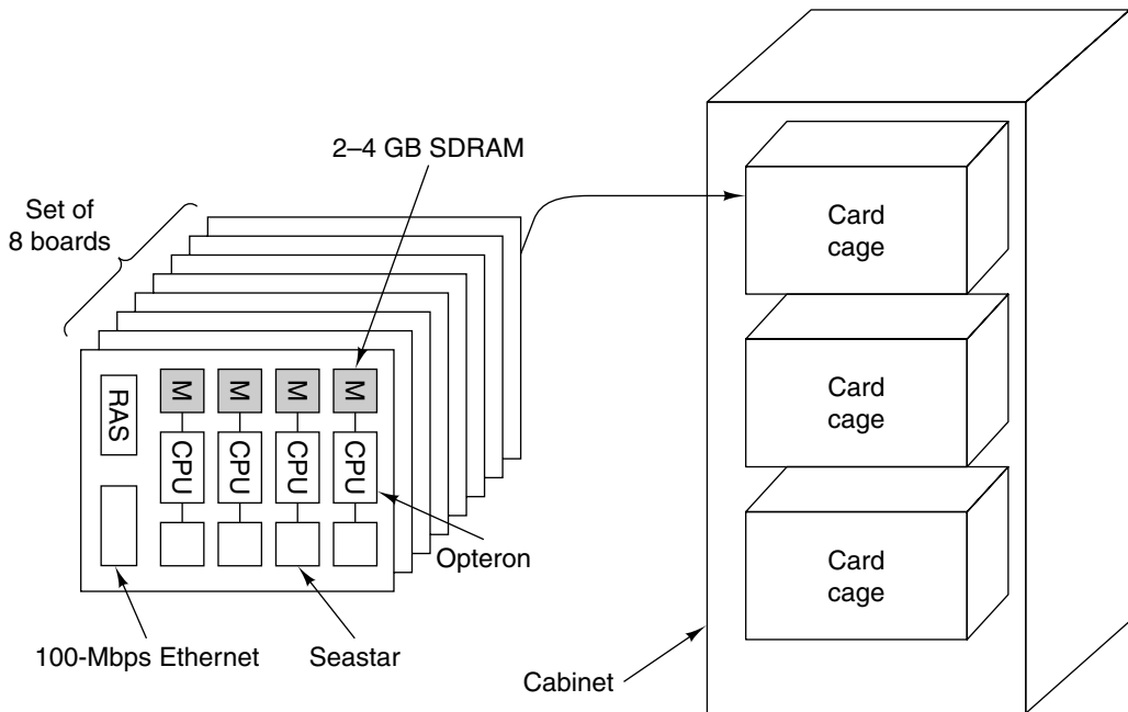
Figure 8-38. Packaging of the Red Storm components.
