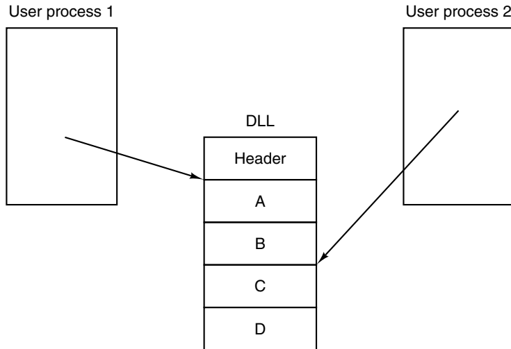
Figure 7-19. Use of a DLL file by two processes.
