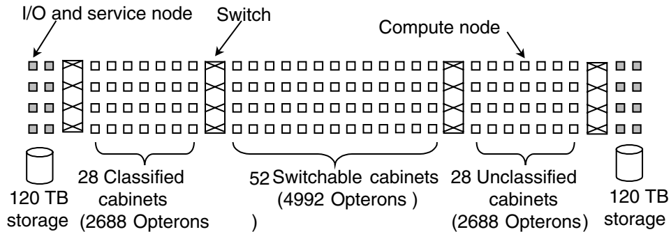
Figure 8-39. The Red Storm system as viewed from above.
