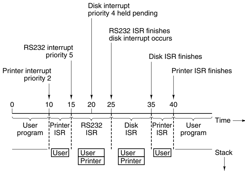
Figure 5-46. Time sequence of multiple interrupt example.
