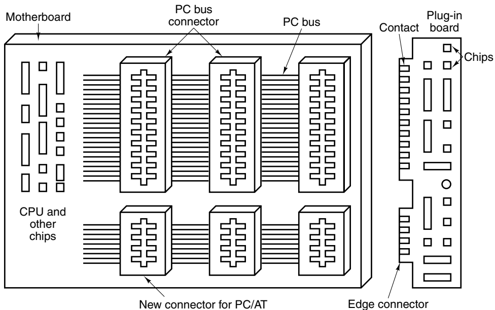
Figure 3-51. The PC/AT bus has two components, the original PC part and the new part.
