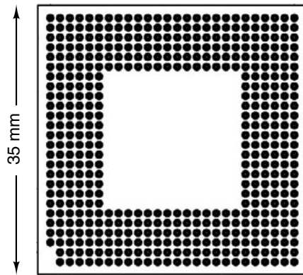
Figure 3-44. The Pentium 4 physical pinout.
