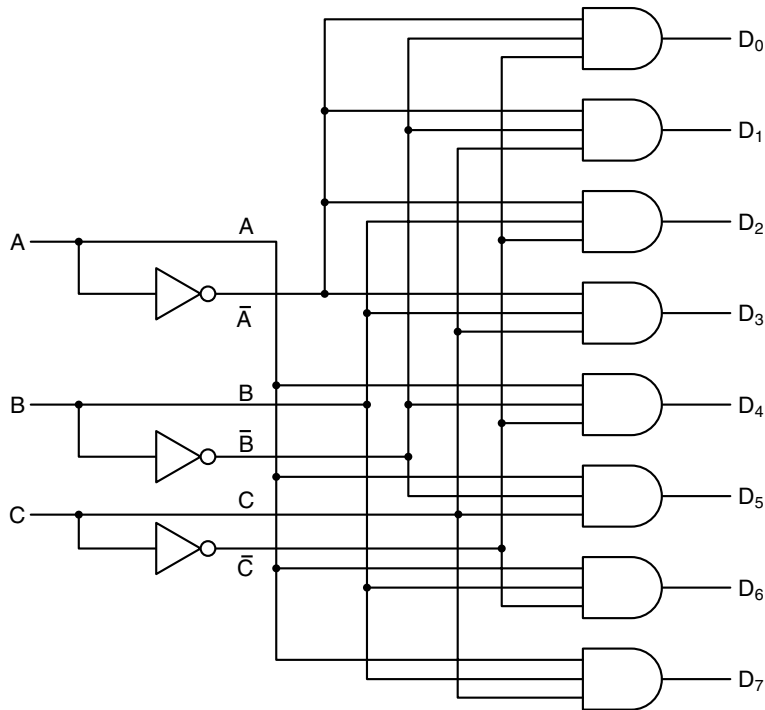
Figure 3-13. A 3-to-8 decoder circuit.
