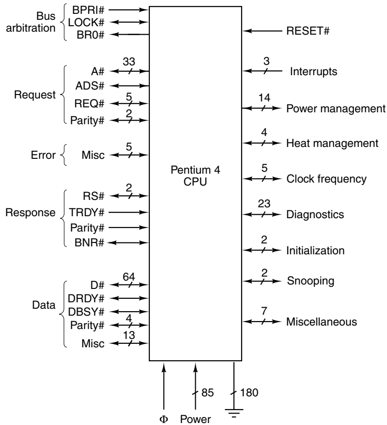
Figure 3-45. Logical pinout of the Pentium 4. Names in uppercase are the official Intel names for individual signals. Names in mixed case are groups of related signals or signal descriptions.
