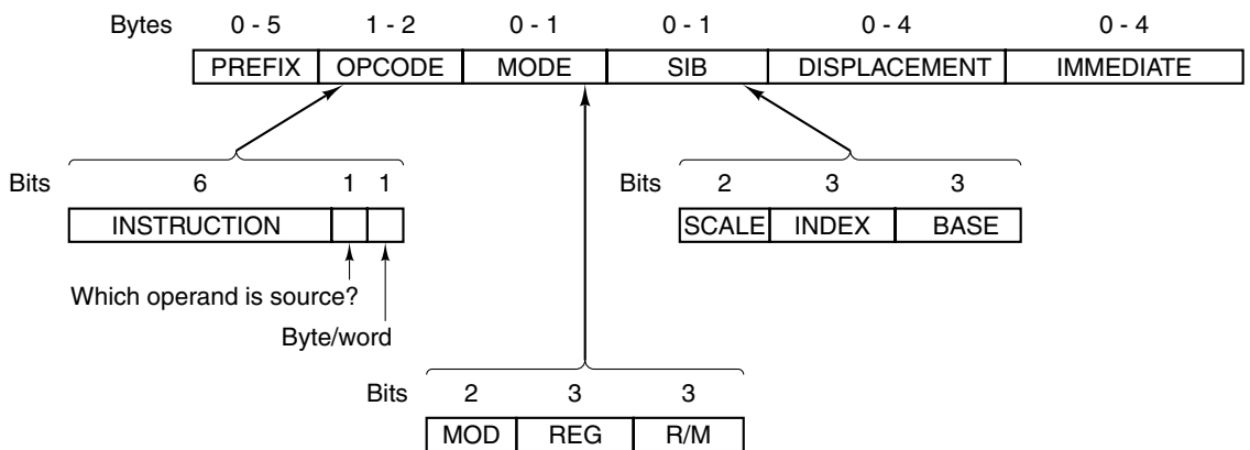
Figure 5-14. The Pentium 4 instruction formats.
