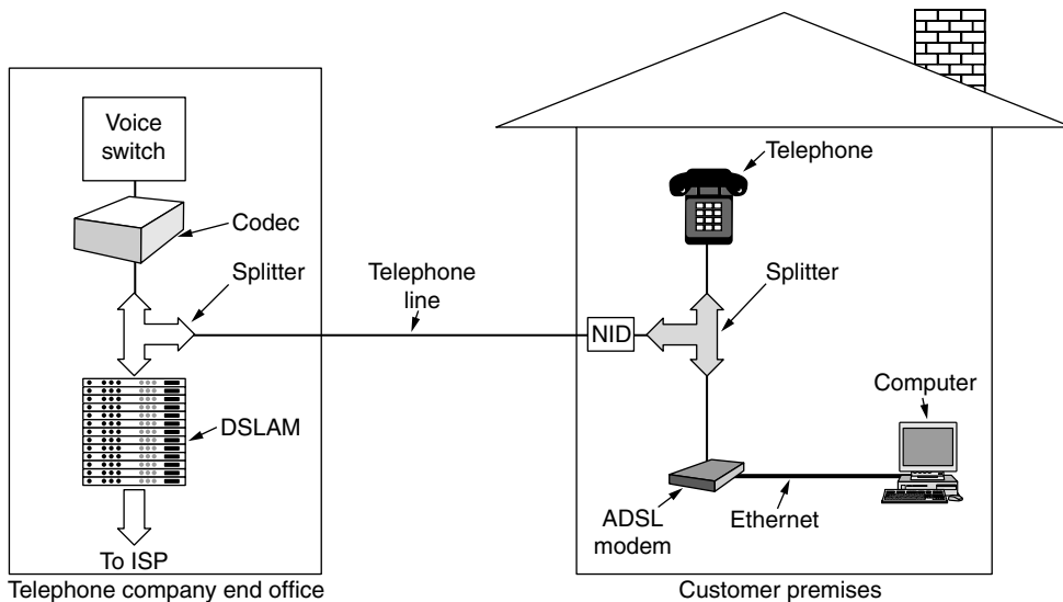
Figure 2-39. A typical ADSL equipment configuration.
