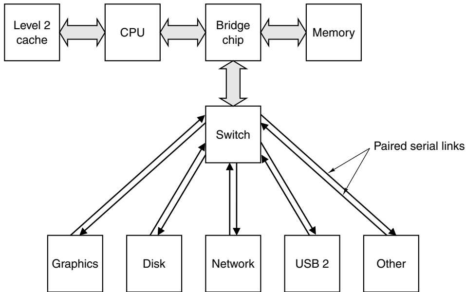
Figure 3-57. A typical PCI Express system.
