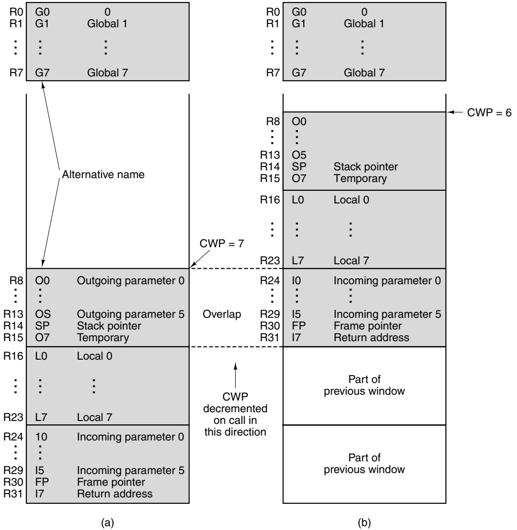
Figure 5-5. Operation of the UltraSPARC III register windows.
