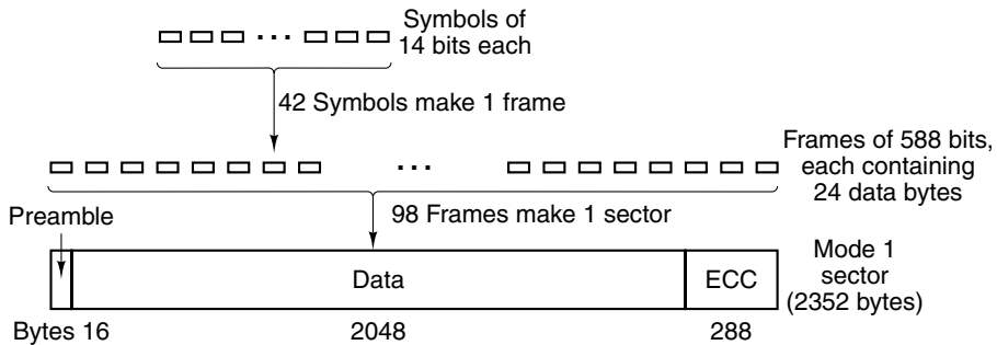
Figure 2-25. Logical data layout on a CD-ROM.
