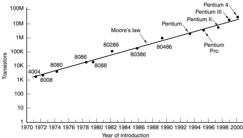
Figure 1-13. Moore's law for (Intel) CPU chips.
