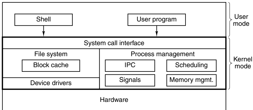
Figure 6-30. The structure of a typical UNIX system.
