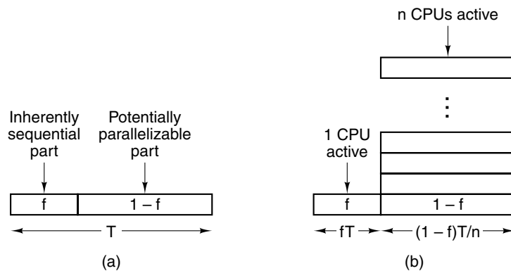
Figure 8-48. (a) A program has a sequential part and a parallelizable part. (b) Effect of running part of the program in parallel.
