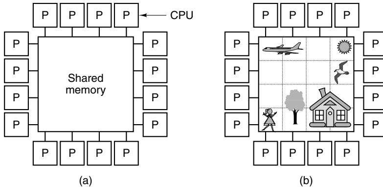
Figure 8-17. (a) A multiprocessor with 16 CPUs sharing a common memory. (b) An image partitioned into 16 sections, each being analyzed by a different CPU.
