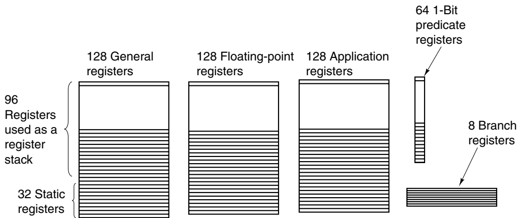
Figure 5-49. The Itanium 2's registers.
