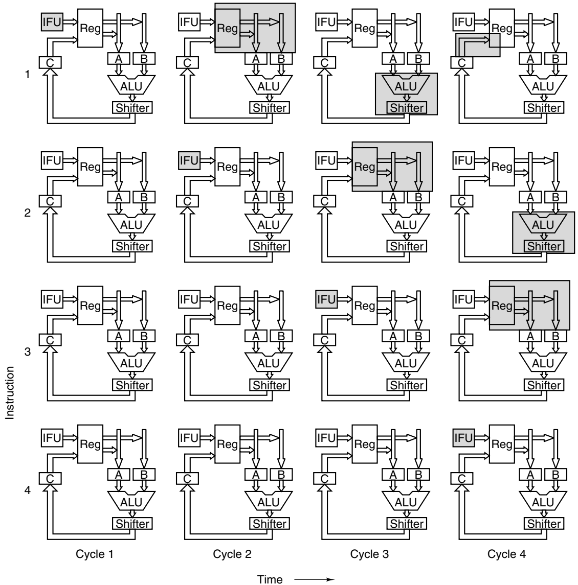
Figure 4-34. Graphical illustration of how a pipeline works.
