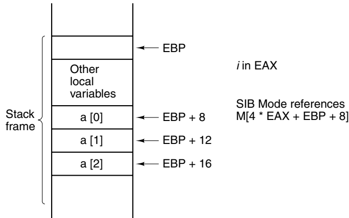
Figure 5-28. Access to a[i] .
