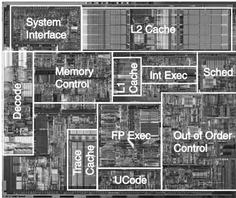
Figure 1-12. The Pentium 4 chip. The photograph is copyrighted by the Intel Corporation, 2003 and used by permission.
