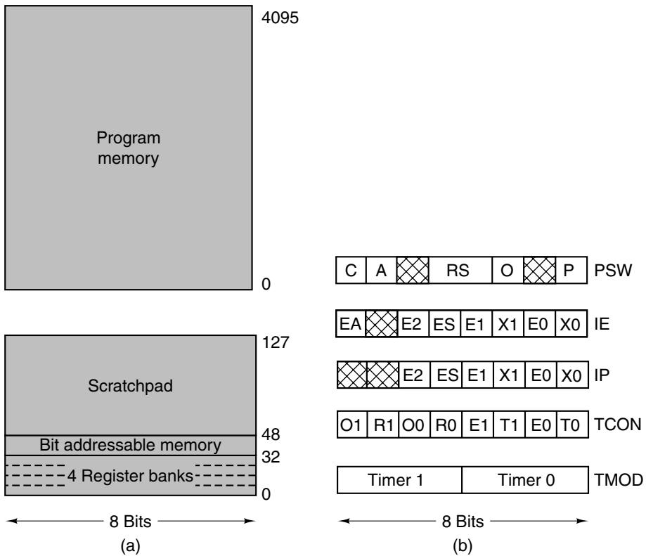
Figure 5-6. (a) On-chip memory organization for the 8051. (b) Major 8051 registers.
