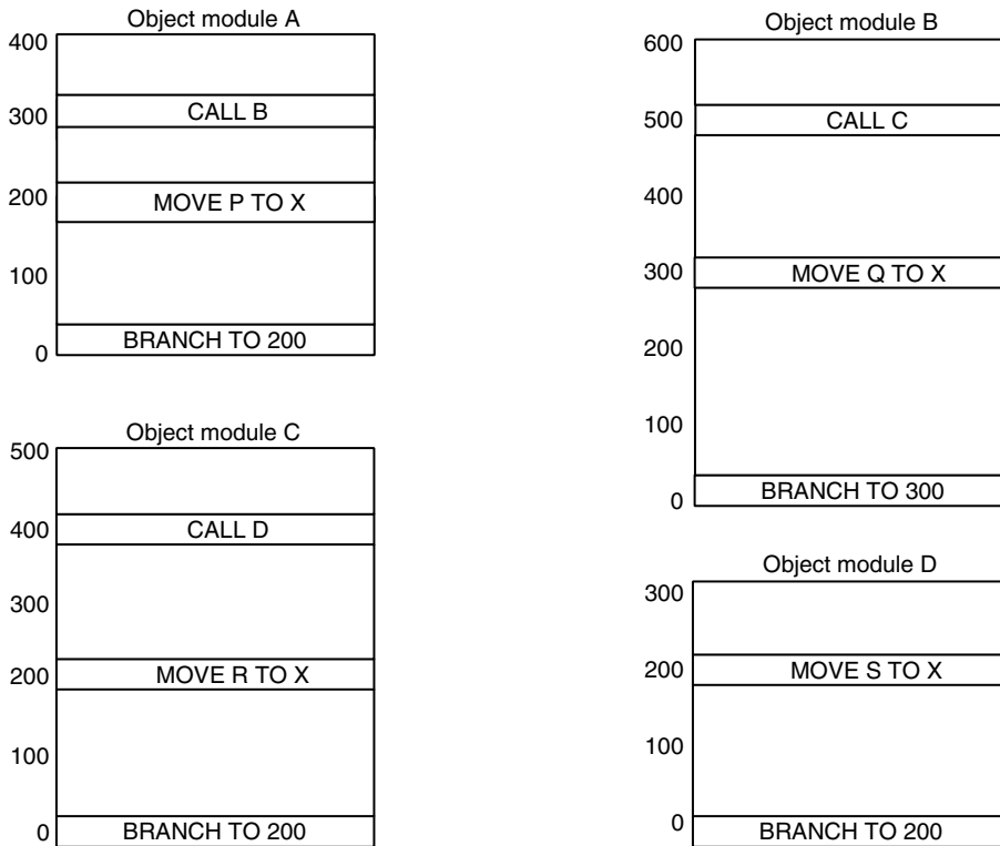
Figure 7-14. Each module has its own address space, starting at 0.
