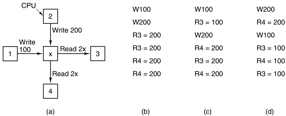
Figure 8-22. (a) Two CPUs writing and two CPUs reading a common memory word. (b) – (d) Three possible ways the two writes and four reads might be interleaved in time.
