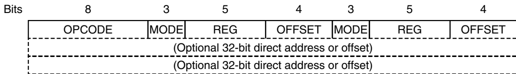
Figure 5-26. A simple design for the instruction formats of a two-address machine.
