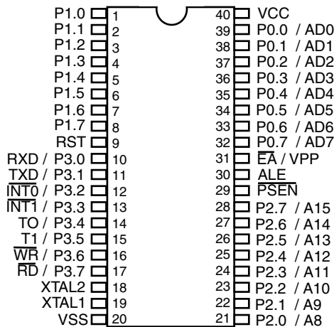
Figure 3-49. Physical pinout of the 8051.
