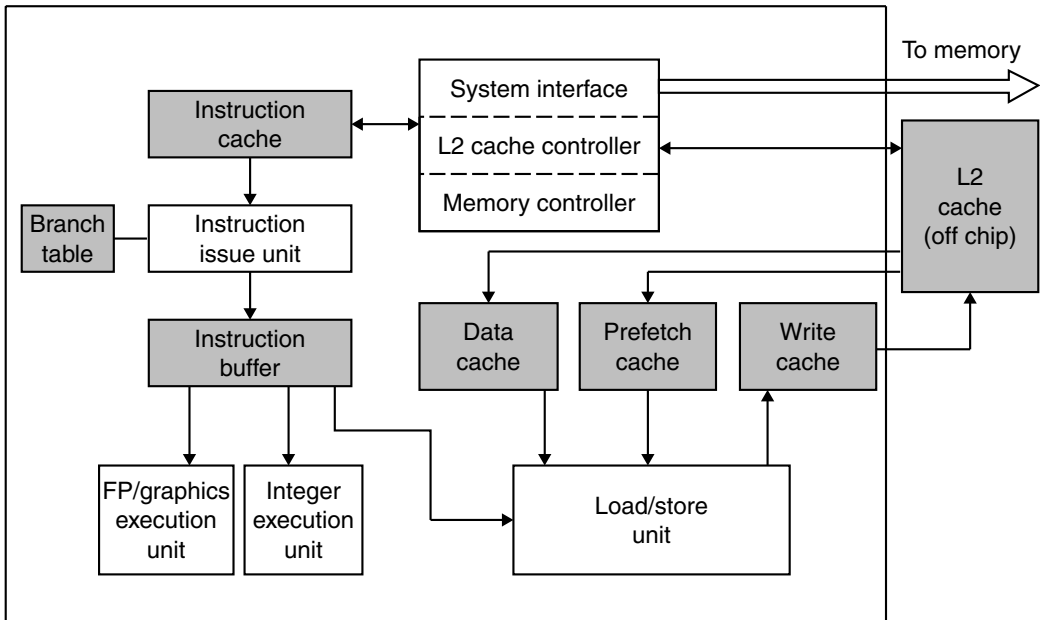
Figure 4-48. The block diagram of the UltraSPARC III Cu.
