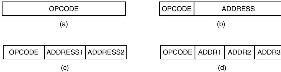
Figure 5-10. Four common instruction formats: (a) Zero-address instruction. (b) One-address instruction (c) Two-address instruction. (d) Three-address instruction.
