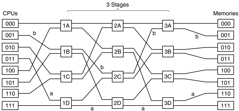
Figure 8-29. An omega switching network.
