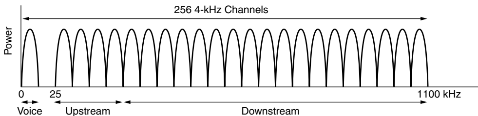
Figure 2-38. Operation of ADSL.
