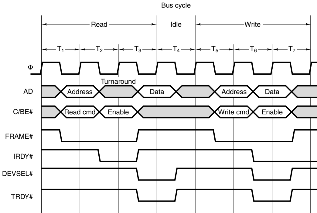
Figure 3-56. Examples of 32-bit PCI bus transactions. The first three cycles are used for a read operation, then an idle cycle, and then three cycles for a write operation.
