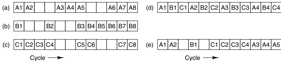
Figure 8-7. (a)–(c) Three threads. The empty boxes indicated that the thread has stalled waiting for memory. (d) Fine-grained multithreading. (e) Coarse-grained multithreading.
