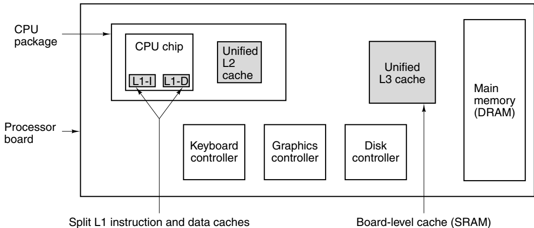
Figure 4-37. A system with three levels of cache.
