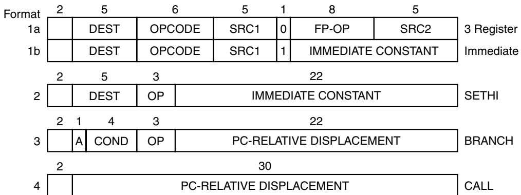
Figure 5-15. The original SPARC instruction formats.
