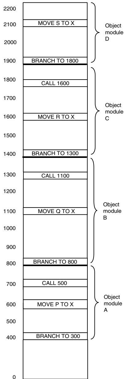
Figure 7-17. The relocated binary program of Fig. 7-15(b) moved up 300 addresses. Many instructions now refer to an incorrect memory address.
