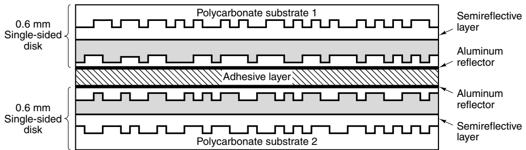
Figure 2-27. A double-sided, dual layer DVD disk.
