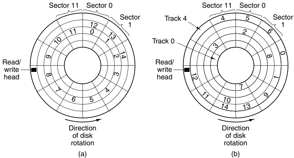
Figure 6-20. Disk allocation strategies. (a) A file in consecutive sectors. (b) A file not in consecutive sectors.
