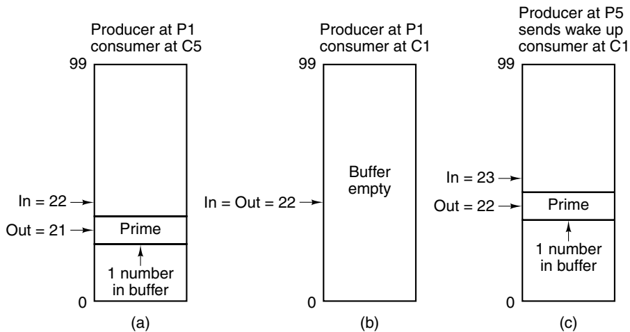
Figure 6-26. Failure of the producer-consumer communication mechanism.
