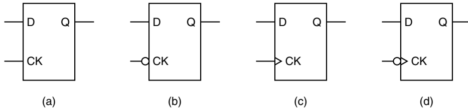
Figure 3-27. D latches and flip-flops.
