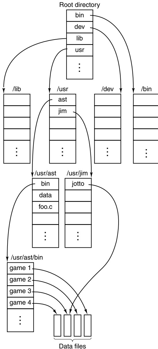
Figure 6-36. Part of a typical UNIX directory system.
