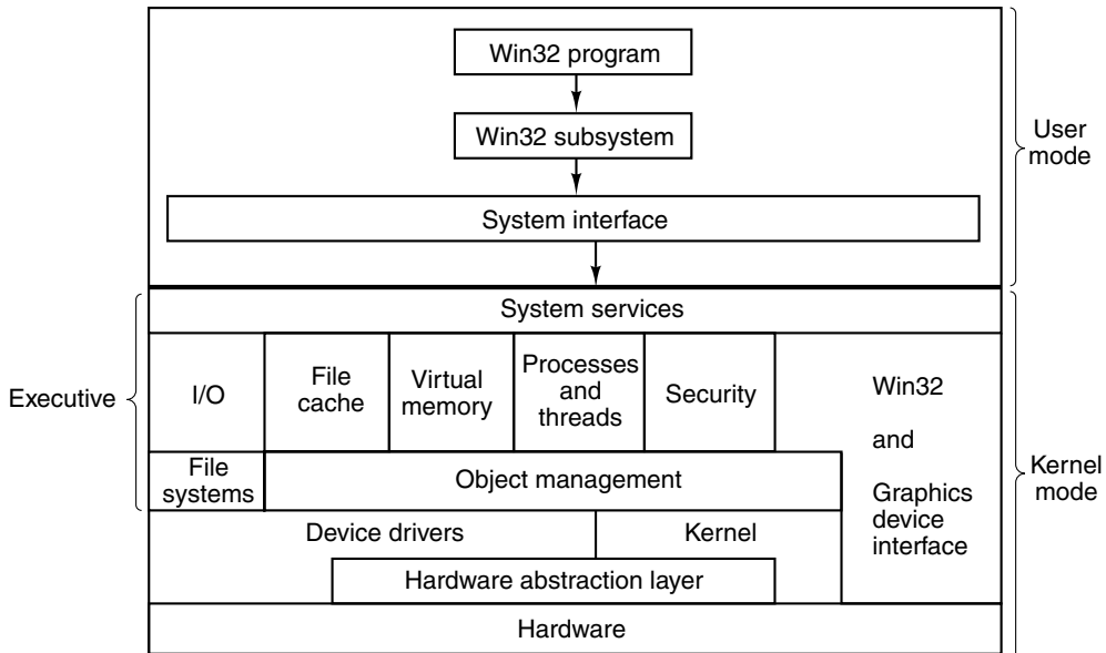
Figure 6-31. The structure of Windows XP.
