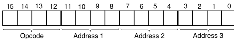
Figure 5-12. An instruction with a 4-bit opcode and three 4-bit address fields.
