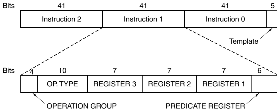
Figure 5-50. An IA-64 bundle contains three instructions.
