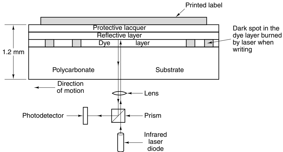
Figure 2-26. Cross section of a CD-R disk and laser (not to scale). A CD-ROM has a similar structure, except without the dye layer and with a pitted aluminum layer instead of a reflective layer.
