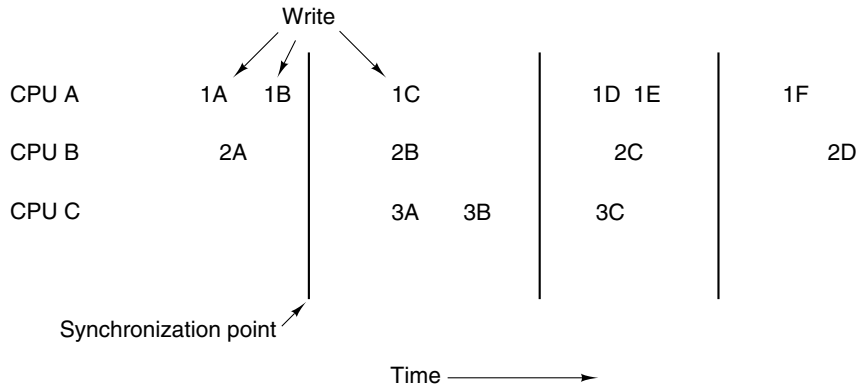
Figure 8-23. Weakly consistent memory uses synchronization operations to divide time into sequential epochs.
