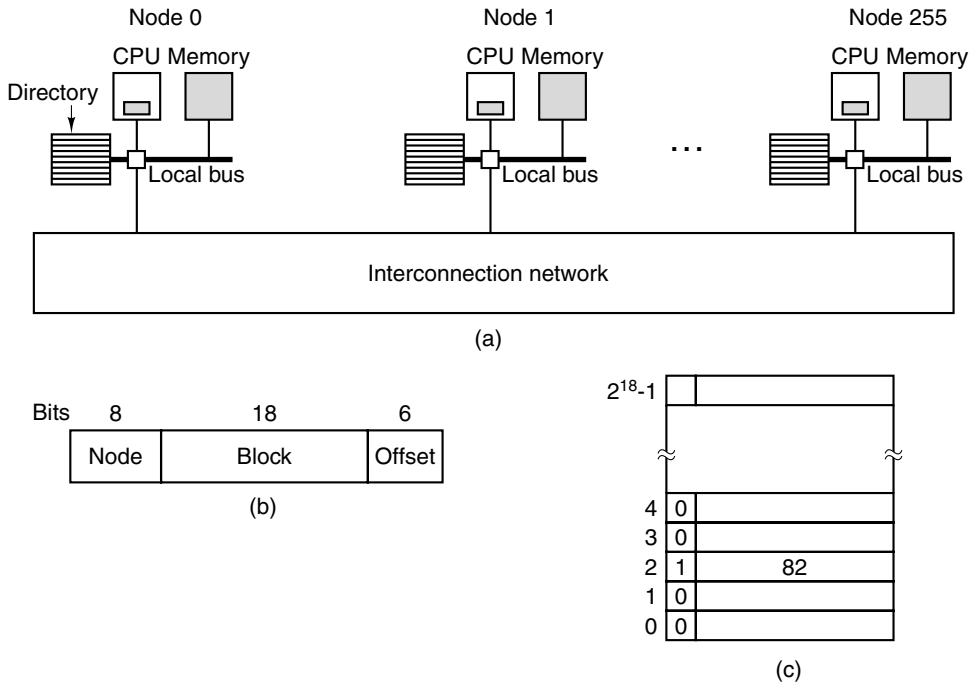
Figure 8-31. (a) A 256-node directory-based multiprocessor. (b) Division of a 32-bit memory address into fields. (c) The directory at node 36.
