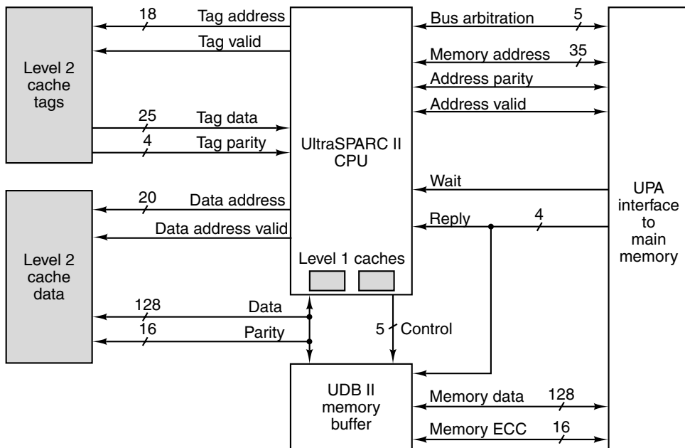
Figure 3-48. The main features of the core of an UltraSPARC III system.
