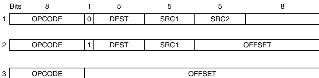
Figure 5-25. A simple design for the instruction formats of a three-address machine.
