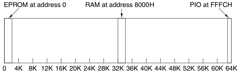
Figure 3-61. Location of the EPROM, RAM, and PIO in our 64 KB address space.
