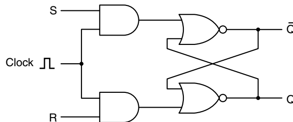
Figure 3-23. A clocked SR latch.
