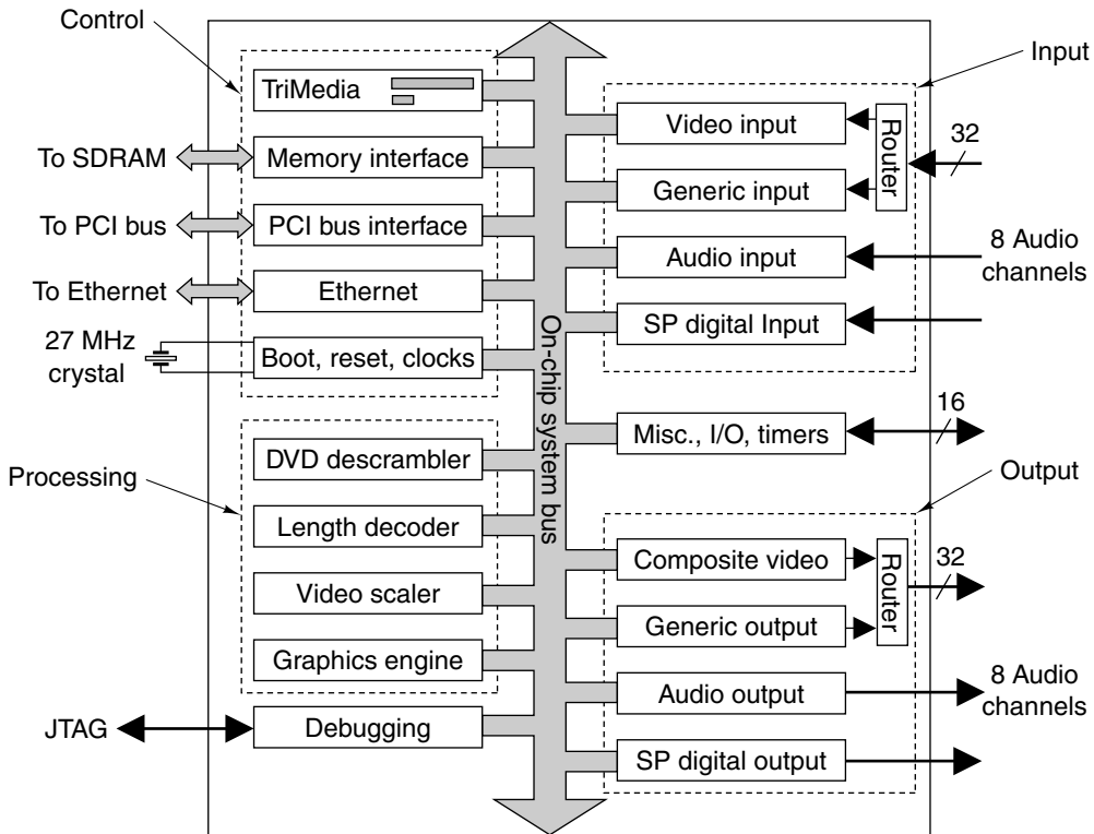
Figure 8-16. The Nexperia heterogeneous multiprocessor on a chip.
