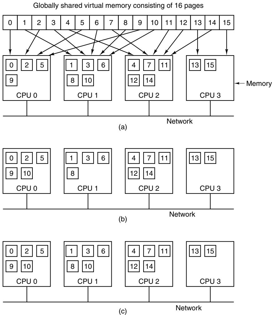
Figure 8-44. A virtual address space consisting of 16 pages spread over four nodes of a multicomputer. (a) The initial situation. (b) After CPU 0 references page 10. (c) After CPU 1 references page 10, here assumed to be a read-only page.
