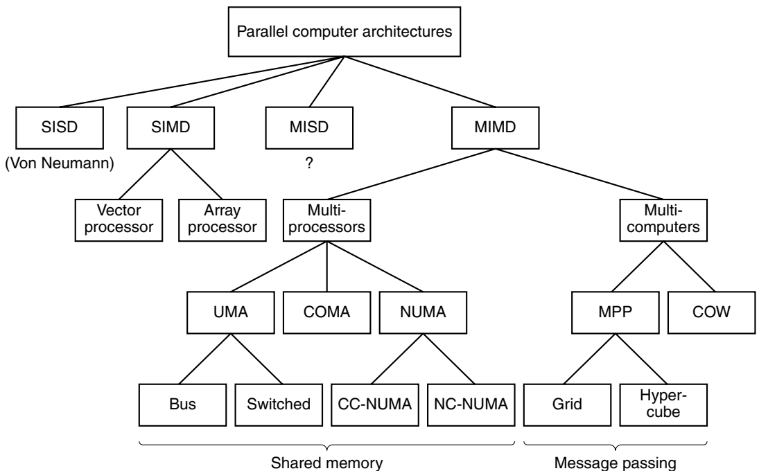
Figure 8-21. A taxonomy of parallel computers.
