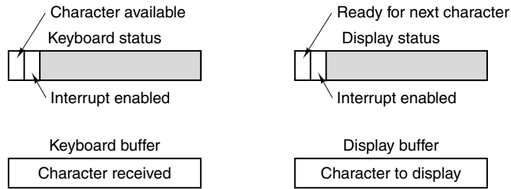
Figure 5-31. Device registers for a simple terminal.
