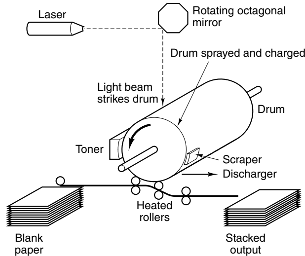
Figure 2-35. Operation of a laser printer.
