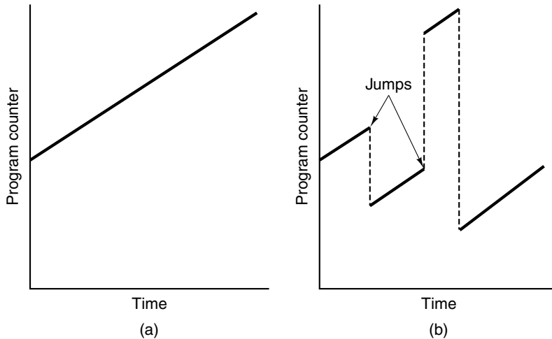
Figure 5-39. Program counter as a function of time (smoothed). (a) Without branches. (b) With branches.
