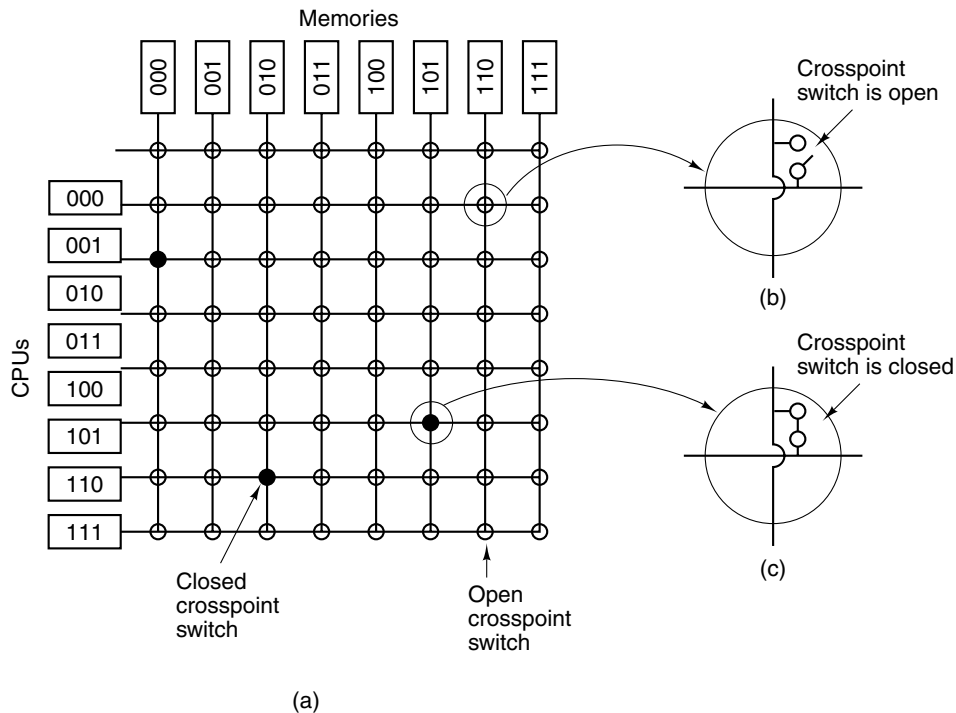
Figure 8-27. (a) An 8 \times 8 crossbar switch. (b) An open crosspoint. (c) A closed crosspoint.
