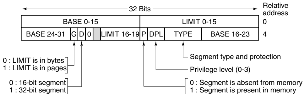
Figure 6-13. A Pentium 4 code segment descriptor. Data segments differ slightly.
