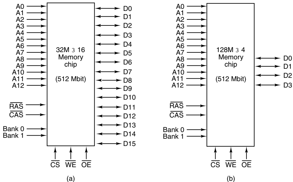
Figure 3-32. Two ways of organizing a 512-Mbit memory chip.
