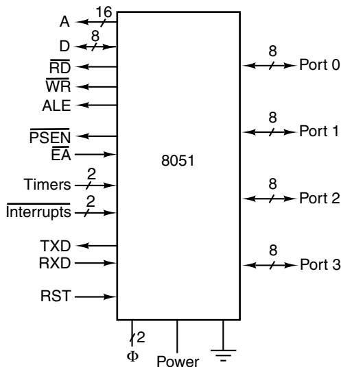
Figure 3-50. Logical pinout of the 8051.
