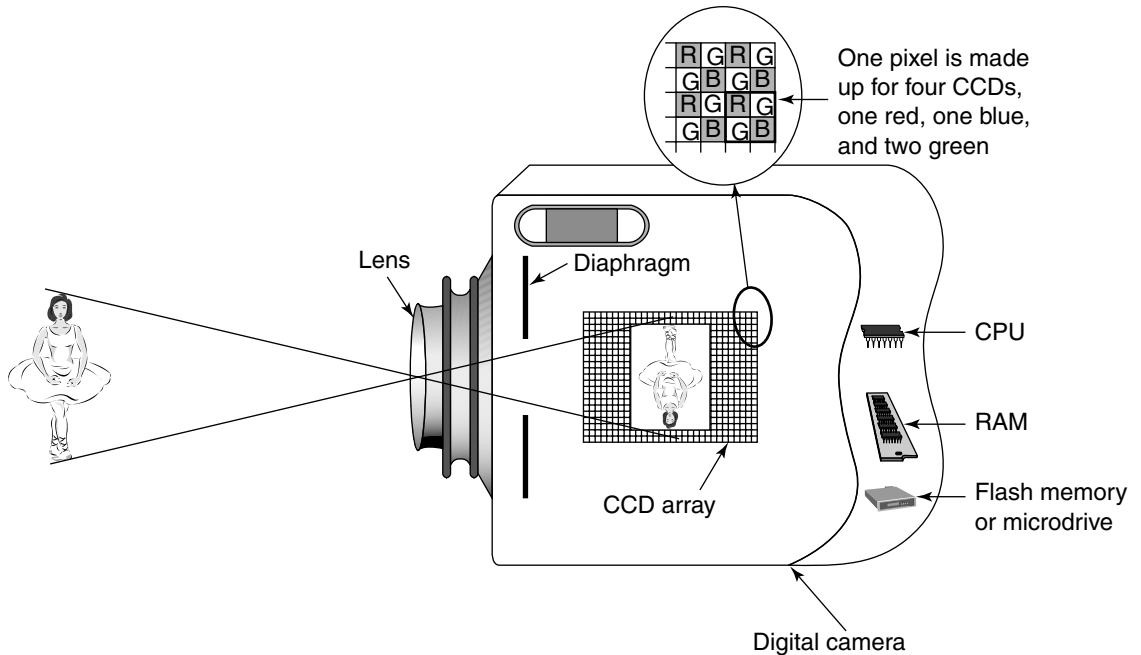
Figure 2-42. A digital camera.
