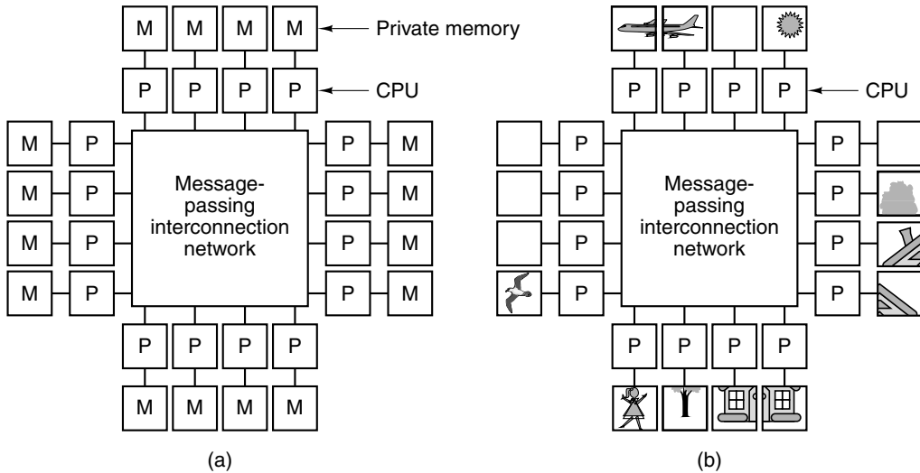
Figure 8-18. (a) A multicomputer with 16 CPUs, each with its own private memory. (b) The bit-map image of Fig. 8-17 split up among the 16 memories.
