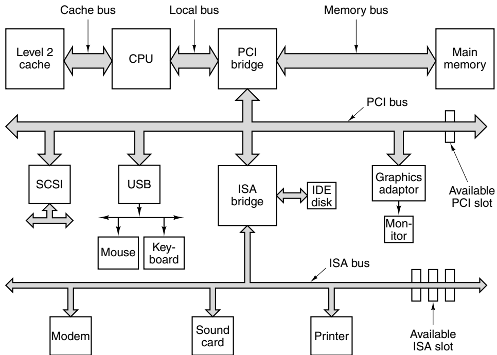
Figure 3-52. Architecture of an early Pentium system. The thicker buses have more bandwidth than the thinner ones but the figure is not to scale.
