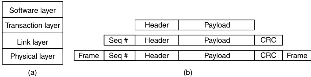
Figure 3-58. (a) The PCI Express protocol stack. (b) The format of a packet.
