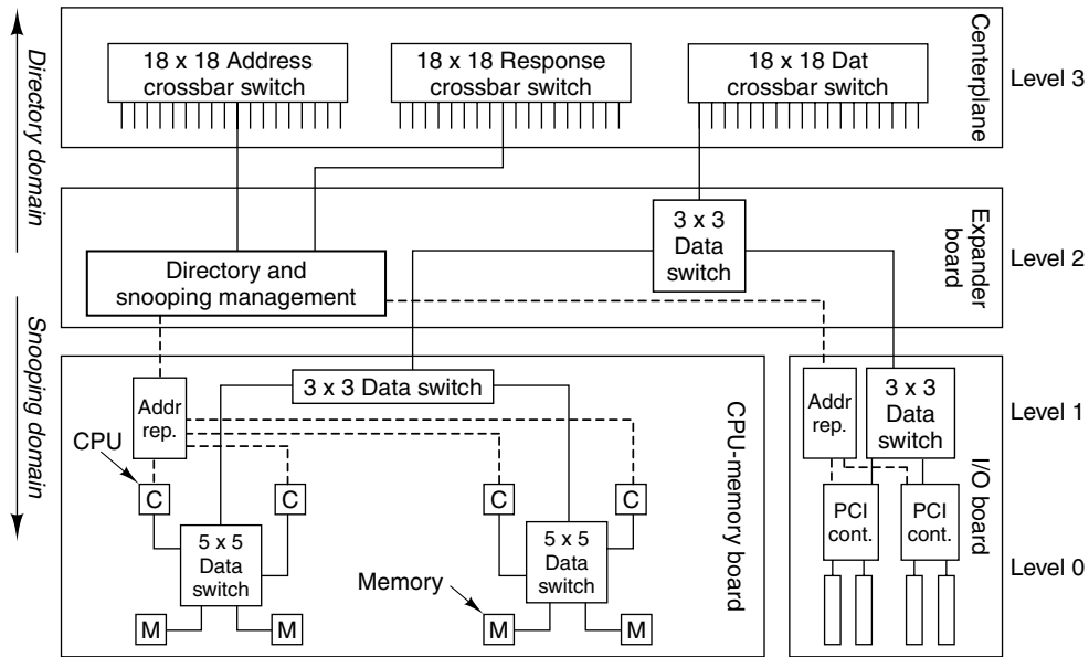
Figure 8-33. The Sun Fire E25K uses a four-level interconnect. Dashed lines are address paths. Solid lines are data paths.
