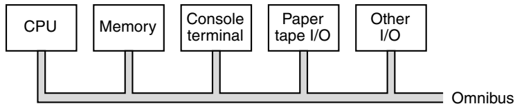
Figure 1-6. The PDP-8 omnibus.
