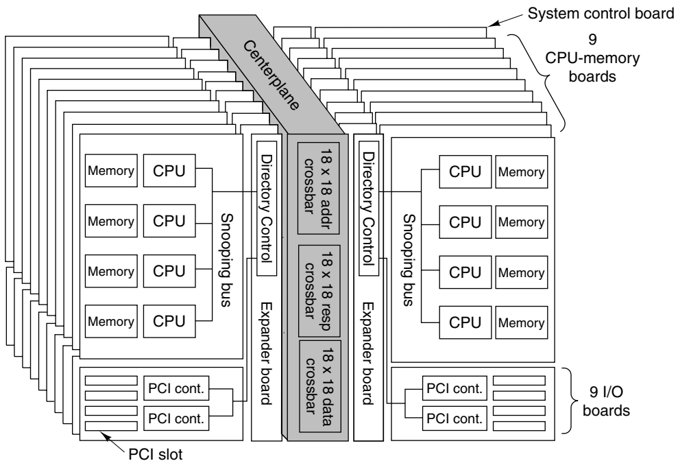
Figure 8-32. The Sun Microsystems E25K multiprocessor.
