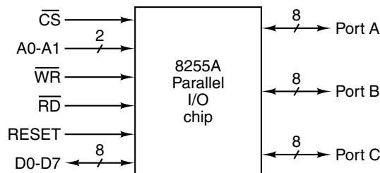
Figure 3-60. An 8255A PIO chip.
