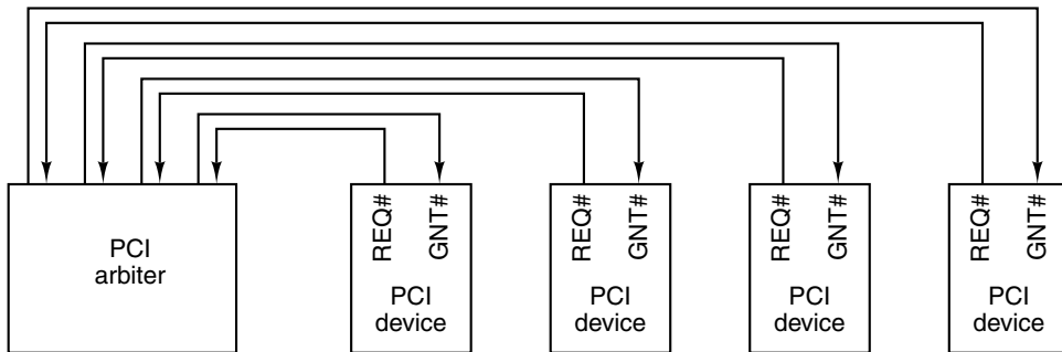
Figure 3-54. The PCI bus uses a centralized bus arbiter.
