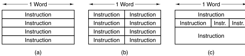
Figure 5-11. Some possible relationships between instruction and word length.
