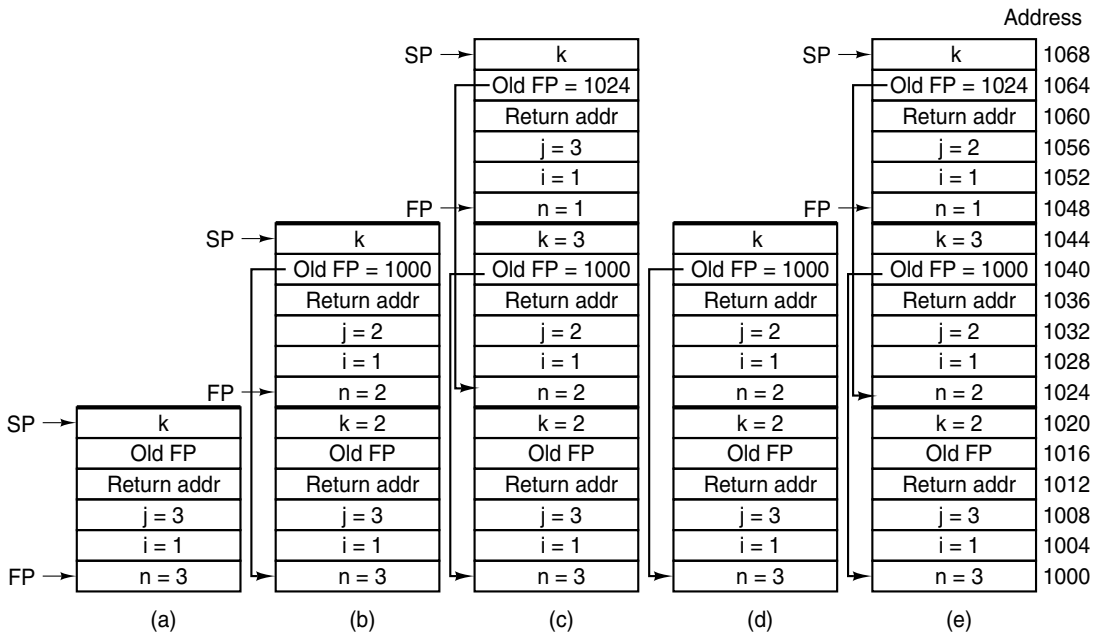
Figure 5-43. The stack at several points during the execution of Fig. 5-42.
