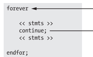
Figure 7-2: continue destination for the forever loop
