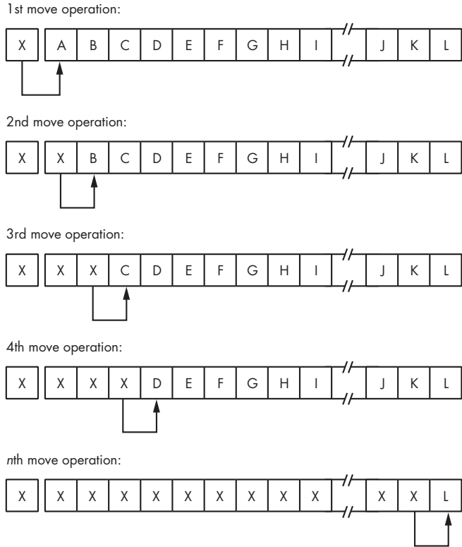
Figure 11-1: Copying data between two overlapping arrays (forward direction)
