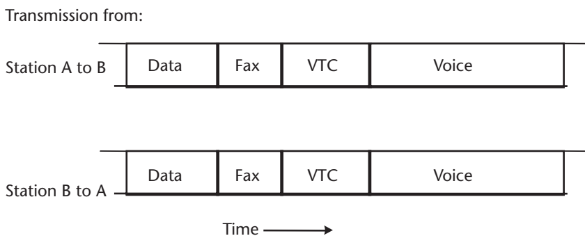
Figure 10.14 Transponder timelines for single destination TDM carriers for a pair of communicating Earth stations.
