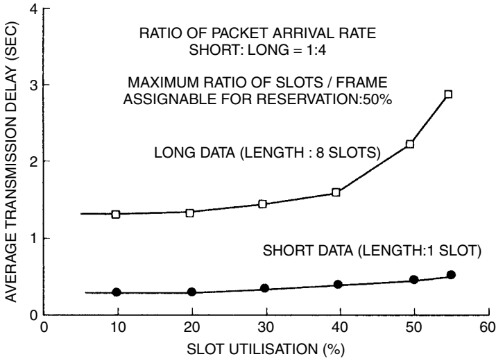
Figure 4.38 Delay versus throughput for mixed mode transmission. (Reproduced from (FUJ86) by permission of the Institute of Electrical and Electronics Engineers, Inc, © 1986 IEEE)
