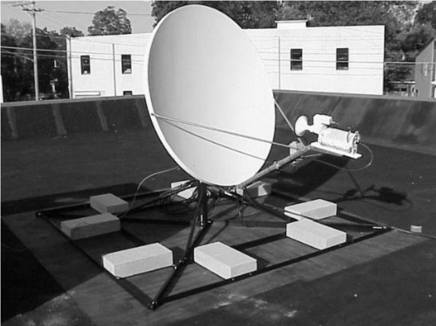
Figure 3.1 Non-penetrating roof mount for VSAT. http://www.freedom-commconsulting.com
