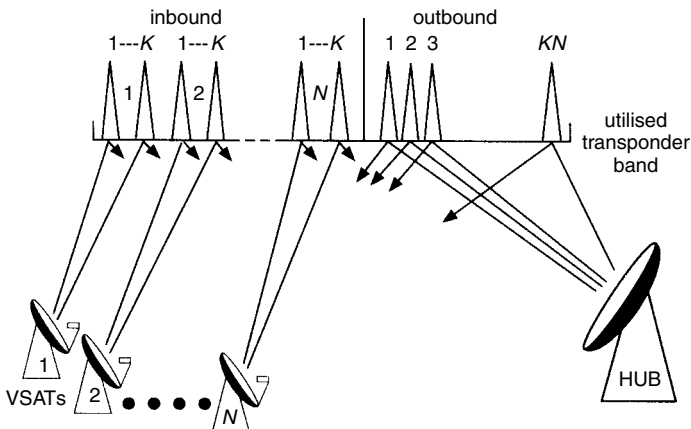
Figure 4.16 Star-shaped network with a two-way connection being conveyed on two SCPC carriers: one from the VSAT to the hub station, and one from the hub to the VSAT. Satellite transponder access is FDMA
