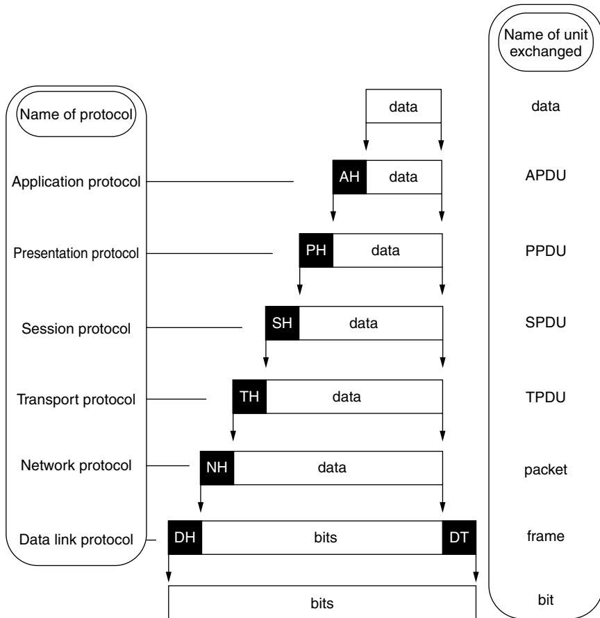
Figure 4.5 Encapsulation from layer to layer in the OSI reference model
