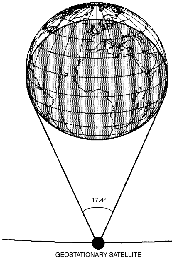
Figure 2.5 Global coverage
