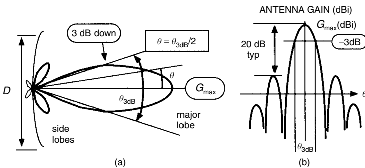
Figure A4.1 Antenna radiation pattern, (a) polar coordinates; (b) Cartesian coordinates (dB on vertical scale)
