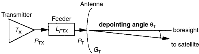
Figure 5.6 Transmitting earth station components
