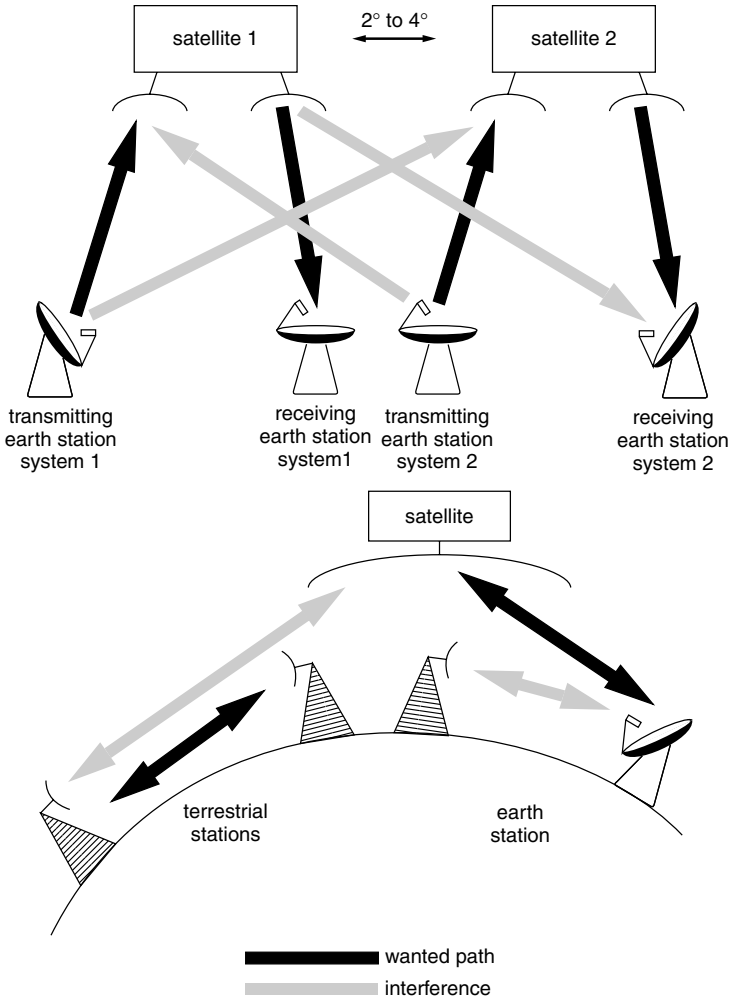
Figure 1.19 Interference paths
