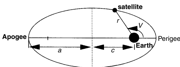
Figure 2.17 Positioning the satellite in its orbit
